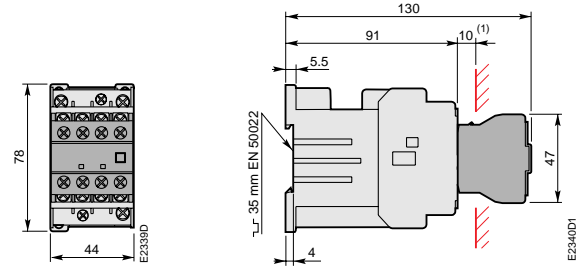
AL 9 ... AL 16 TAL 9 ... TAL 16 NL., TNL.. + CA 5 front-mounted 4-pole auxiliary contact block
