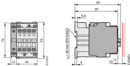
AL 9 ... AL 16 TAL 9 ... TAL 16 NL., TNL.. + CAL 5 side-mounted 2-pole auxiliary contact block
