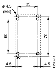
AL 9 ... AL 16, AL..Z. TAL 9 ... TAL 16 NL., NL Z., TNL.. drilling plan
