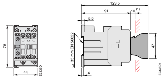
AL 9 ... AL 16, AL..Z. TAL 9 ... TAL 16 NL., NL Z., TNL.. + CA 5 front-mounted 1-pole auxiliary contact block
